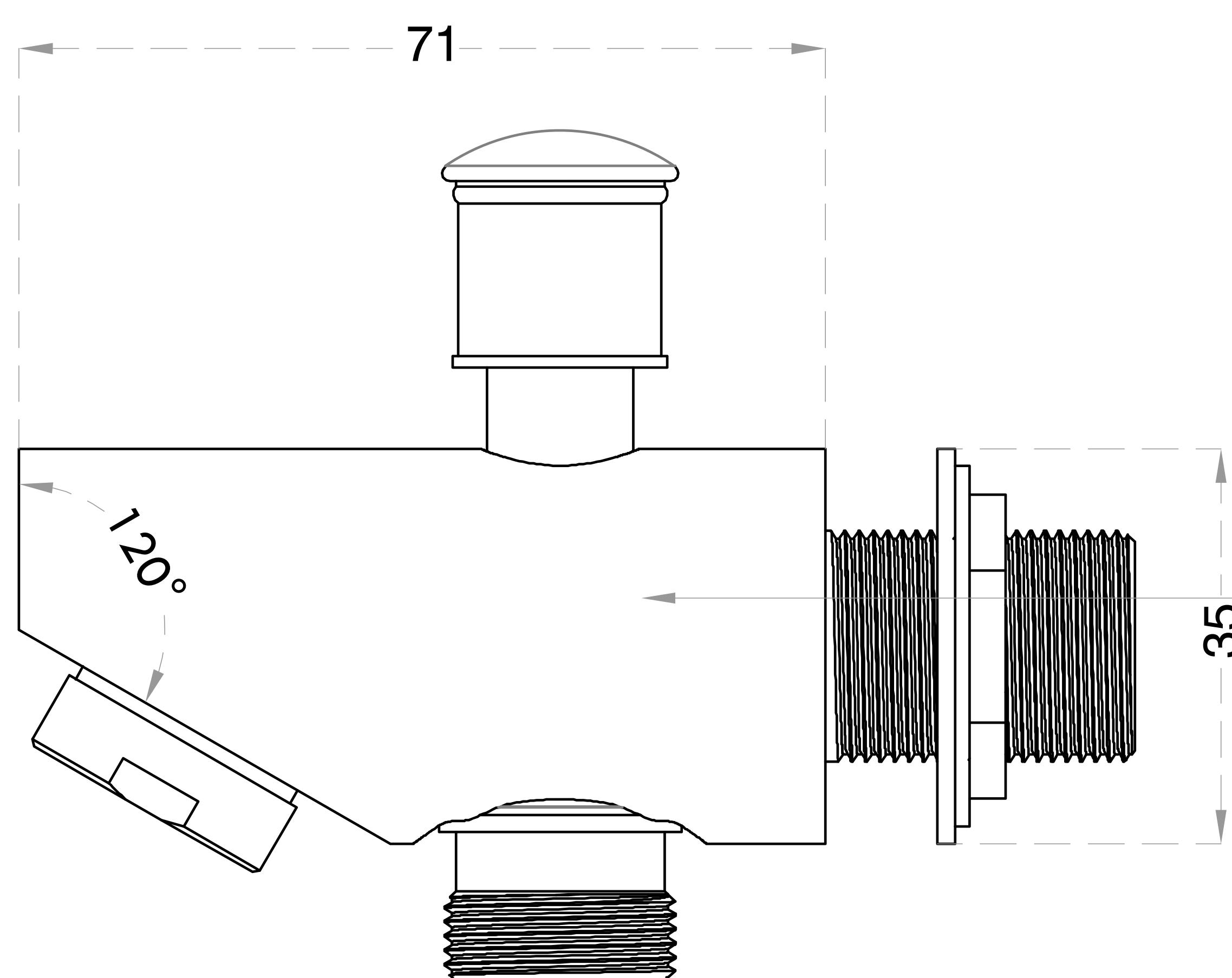
SIDE ELEVATION
