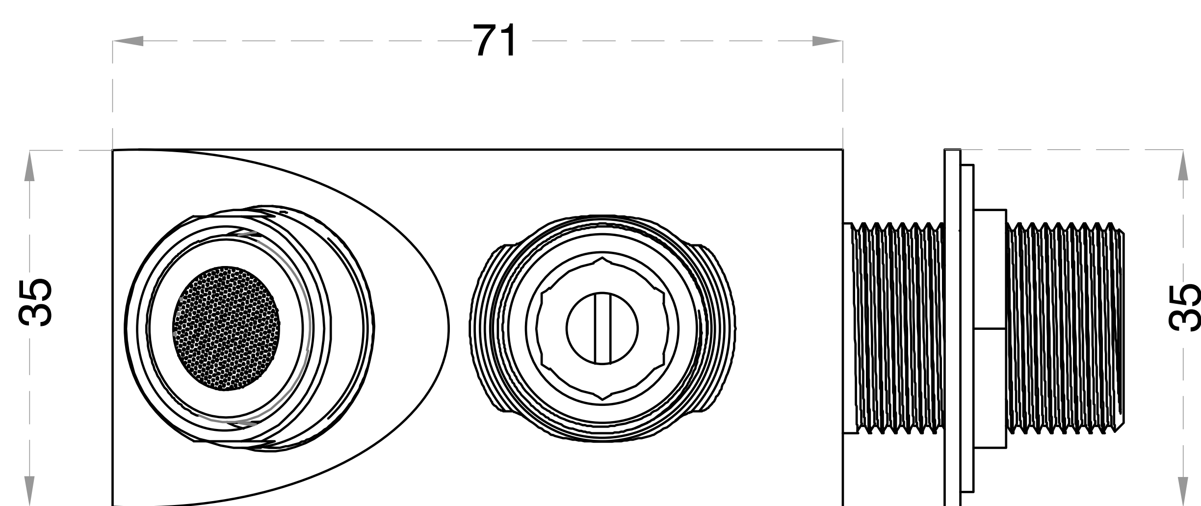
PLAN
