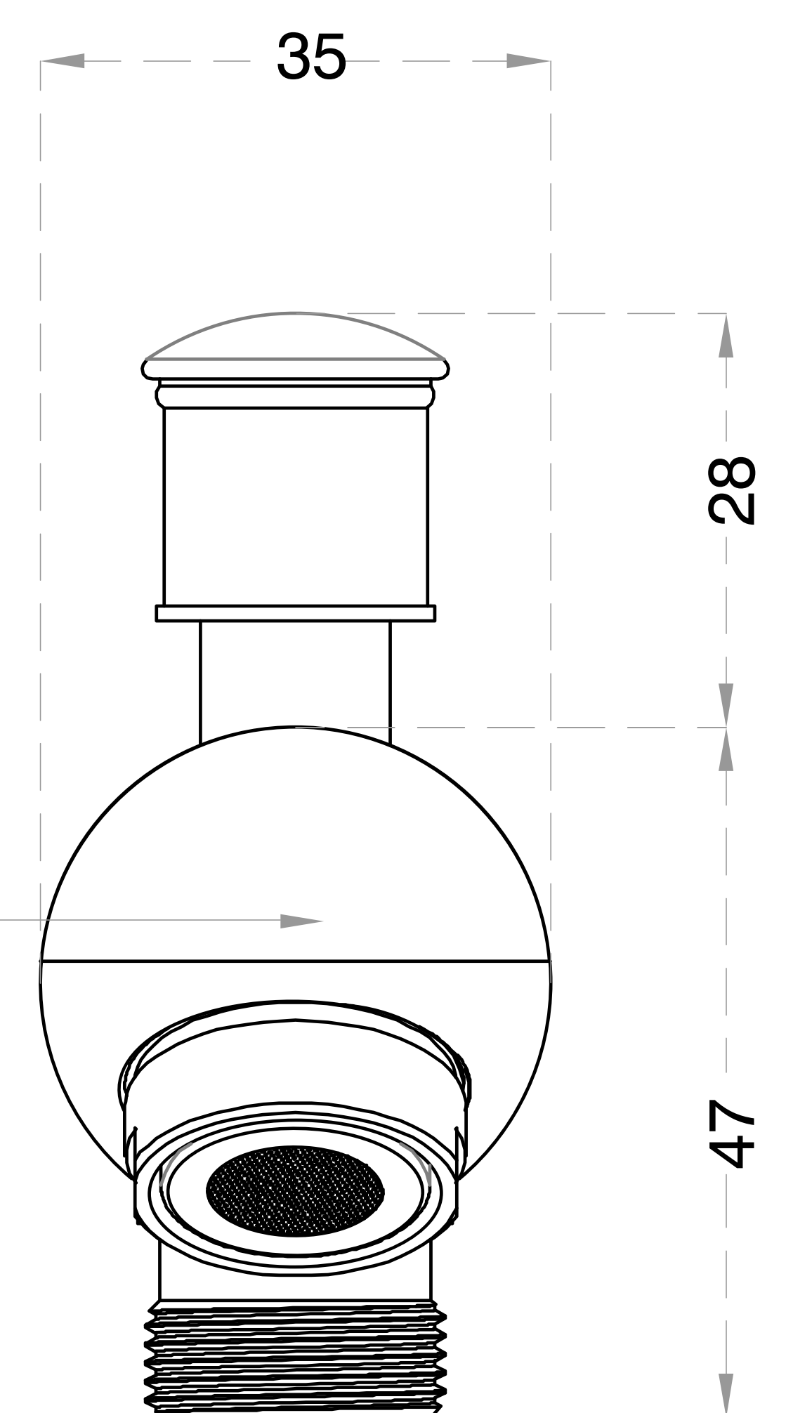
FRONT ELEVATION
